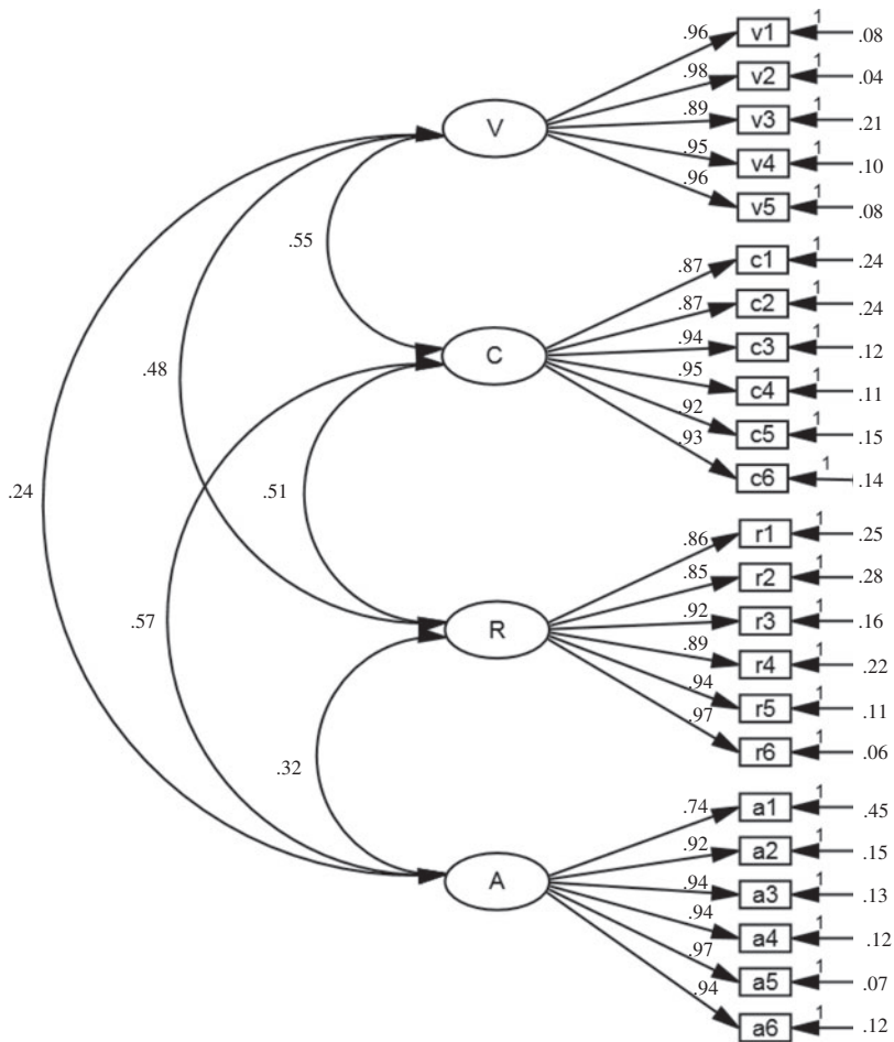
Figure 1. CFA model, interfactor correlations, standardized factor loadings and residuals. Note: n = 367 . All correlations have p < .01 . V = Variety, C = Competence, R = Relatedness, A = Autonomy.
