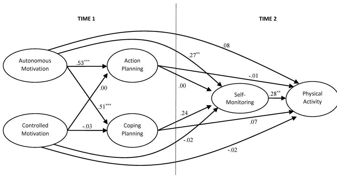
Figure 2 — Standardized parameter estimates of a structural equation model of effects among motivation, planning, self-monitoring, leisure-time physical activity, and demographic variables. Statistically significant indirect effects not shown in model: Autonomous motivation → Physical activity ( \beta = .08 , p = .050 ); Autonomous motivation → Self-monitoring ( \beta = .12 , p = .021 ). Effects of gender, school, and past physical activity behavior as control variables on each variable in the model omitted for clarity, paths freely estimated but not depicted in diagram: Gender → Autonomous motivation ( \beta = .05 , p = .458 ); Gender → Controlled motivation ( \beta = -.19 , p = .026 ); Gender → Action planning ( \beta = -.13 , p = .025 ); Gender → Coping planning ( \beta = -.24 , p < .001 ); Gender → Self-monitoring ( \beta = .04 , p = .490 ); Gender → Physical activity ( \beta = -.14 , p = .054 ); School → Autonomous motivation ( \beta = -.02 , p = .771 ); School → Controlled motivation ( \beta = .023 , p = .78 ); School → Action planning ( \beta = -.09 , p = .097 ); School → Coping planning ( \beta = -.10 , p = .097 ); School → Self-monitoring ( \beta = .13 , p = .032 ); School → Physical activity ( \beta = -.02 , p = .757 ); Past physical activity behavior → Autonomous motivation ( \beta = .46 , p < .001 ); Past physical activity behavior → Controlled motivation ( \beta = -.10 , p = .307 ); Past physical activity behavior → Action planning ( \beta = .21 , p = .002 ); Past physical activity behavior → Coping planning ( \beta = .22 , p = .004 ); Past physical activity behavior → Self-monitoring ( \beta = .20 , p = .007 ); Past physical activity behavior → Physical activity ( \beta = .31 , p < .001 ). * p < .05 ** p < .01 *** p < .001 .
