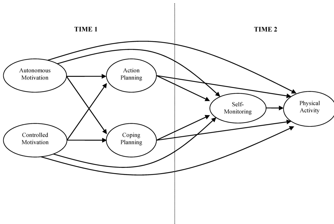
Figure 1 — Proposed structural equation model illustrating effects among self-determination theory, planning, self-monitoring, and behavioral variable. Effects of gender, school, and past physical activity behavior as control variables on each variable in the model omitted for clarity.
