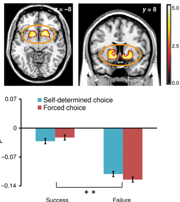
Figure 4. Bilateral striatum activation (peak at 21, 14, -5, and -12, 8, -8) showing a significant main effect of outcome feedback ( P < 0.05 , familywise error corrected; the image is shown at P < 0.001 , uncorrected). Neural responses are displayed in transaxial and coronal formats. The bottom panel represents the mean \beta values (a 6-mm sphere centered on the peak) and corresponding SEs in the striatum as a function of choice condition (self-determined choice vs. forced choice) and outcome feedback (success vs. failure). Note that the graph plotted the activation in the right striatum to allow for reasonable comparison with Figure 5. The plot indicated that the striatum was strongly influenced by outcome feedback (positive vs. negative), but this effect was not modulated by choice condition.
